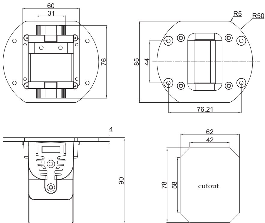
Mechanical drawing
