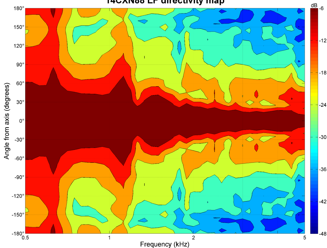
14CXN88 LF directivity map
