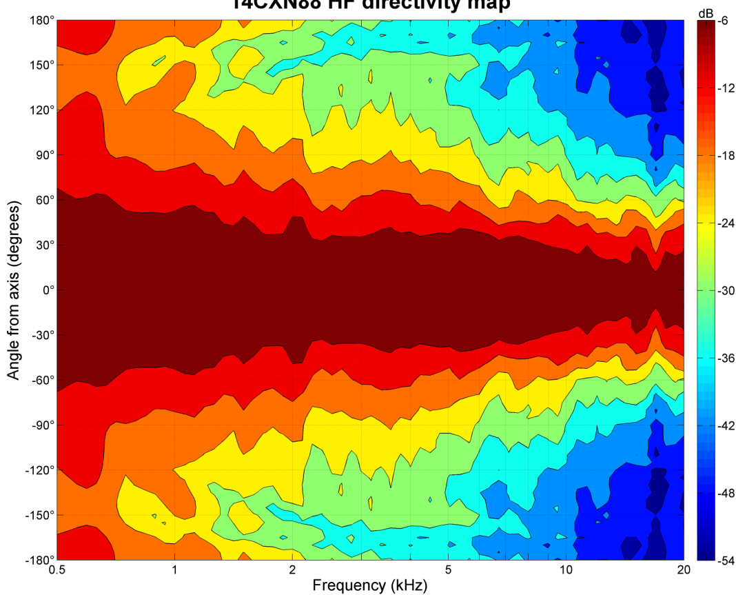
14CXN88 HF directivity map
