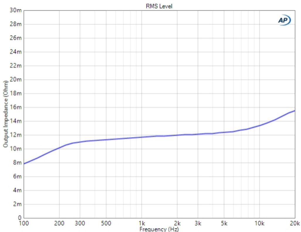
Figure 7: Measured voltage at output terminals while feeding 1A_{RMS} into the output of the amplifier at PCB.
