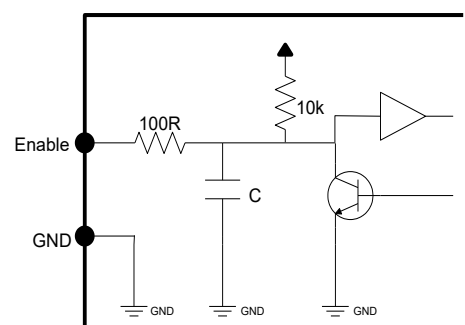
Figure 11: Enable pin interface
