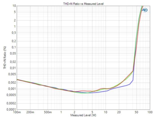
THD+N vs. Po at 100Hz(Blue), 1kHz(Green) and 6.67kHz(Red) 8) (4Ω),
