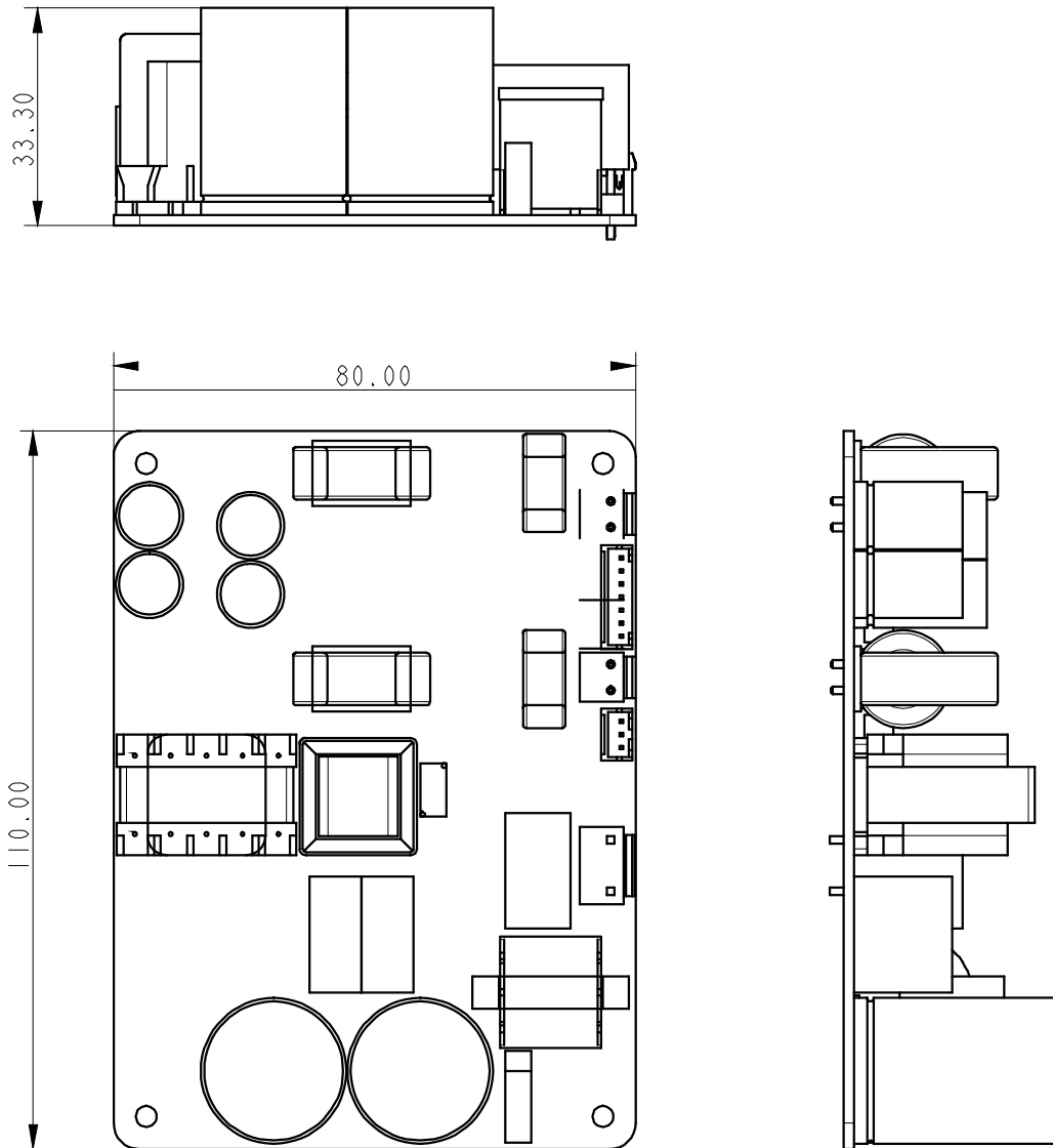
Figure 19: Physical dimensions in mm.
