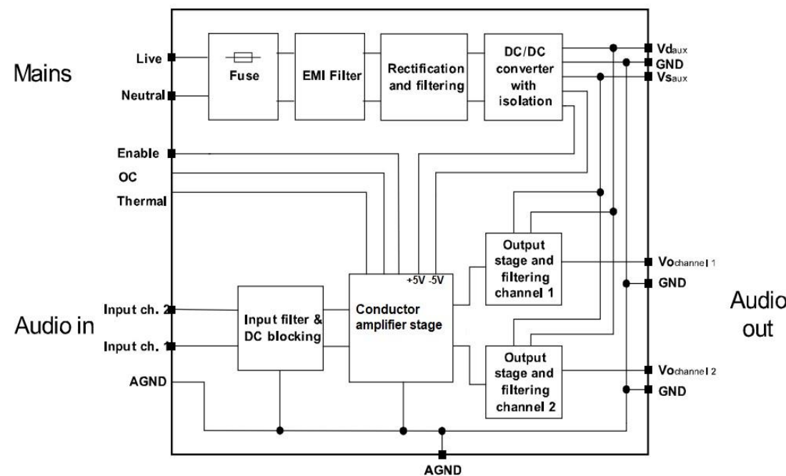
Figure 1: ICEpower50ASX2 block diagram
