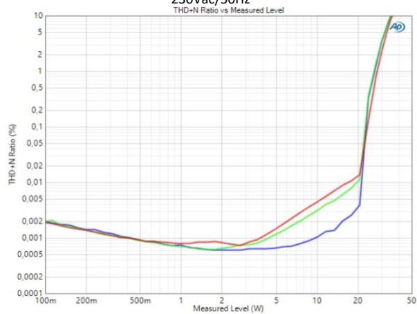
THD+N vs. Po at 100Hz(Blue), 1kHz(Green) and 6.67kHz(Red) 8) (8Ω),
