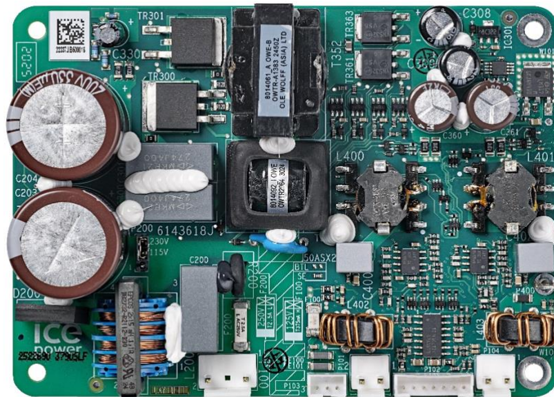
ICEpower50ASX2
