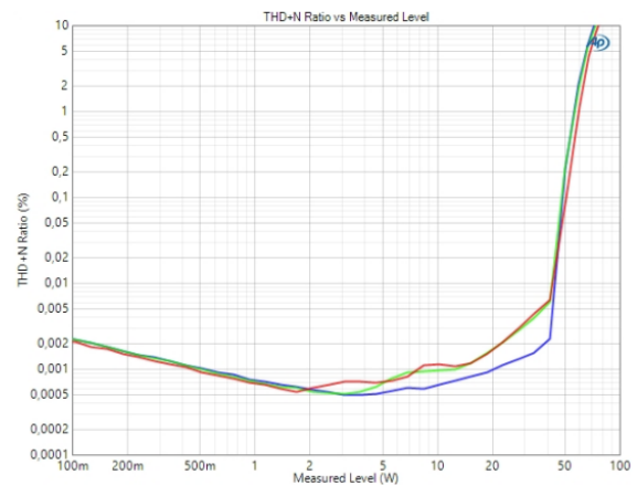
THD+N vs. Po at 100Hz(Blue), 1kHz(Green) and 6.67kHz(Red) 8) (4Ω), 230Vac/50Hz
