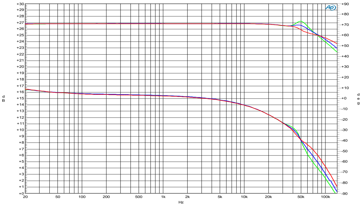
Figure 4: Frequency response in 4Ω (green), 8Ω (blue) and open load (red). Top – amplitude. Bottom – phase.
