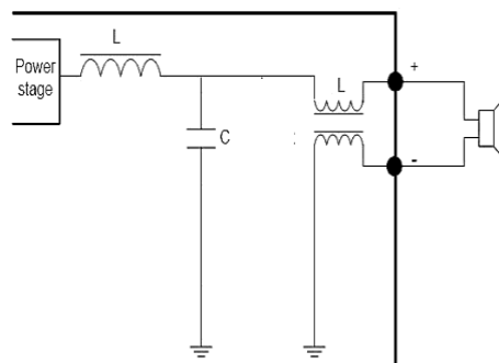
Figure 16: SE output filter section
