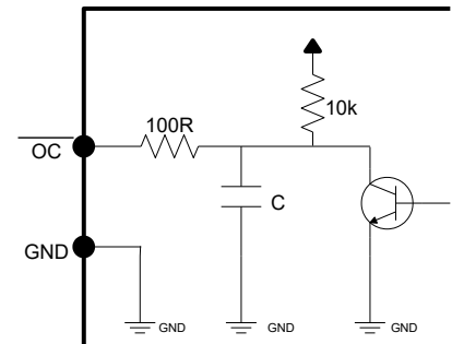
Figure 9: Over Current monitor pin interface
