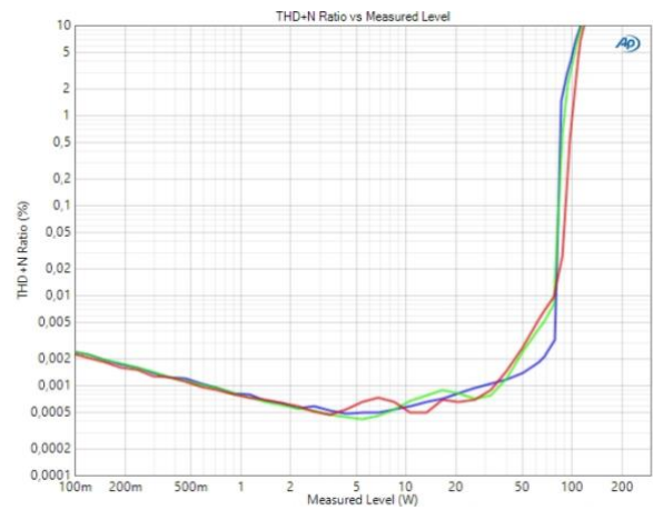
THD+N vs. Po at 100Hz(Blue), 1kHz(Green) and 6.67kHz(Red) 9) (8Ω), 115Vac/50Hz
