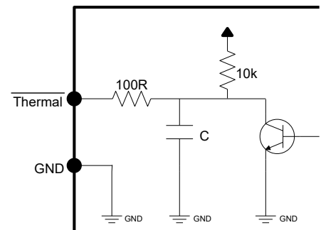
Figure 10: Thermal monitor pin interface
