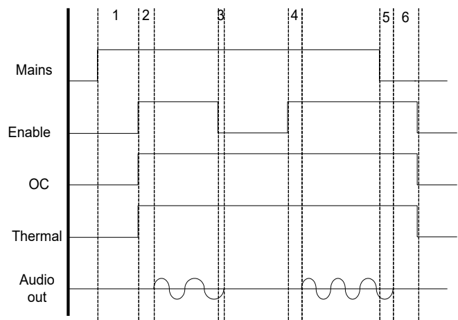
Figure 18: Timing – enable and mains
