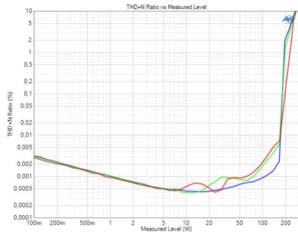
THD+N vs. Po at 100Hz(Blue), 1kHz(Green) and 6.67kHz(Red) 9) (4Ω), 230Vac/50Hz
