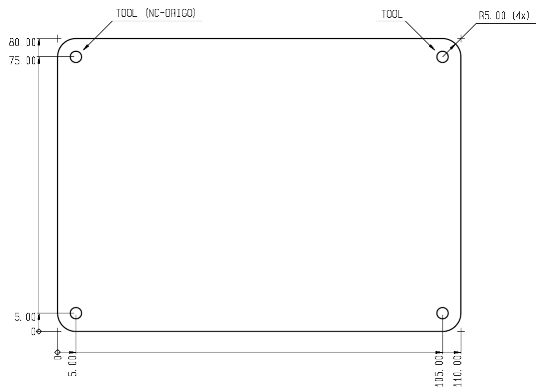
Figure 21: PCB drill pattern.
