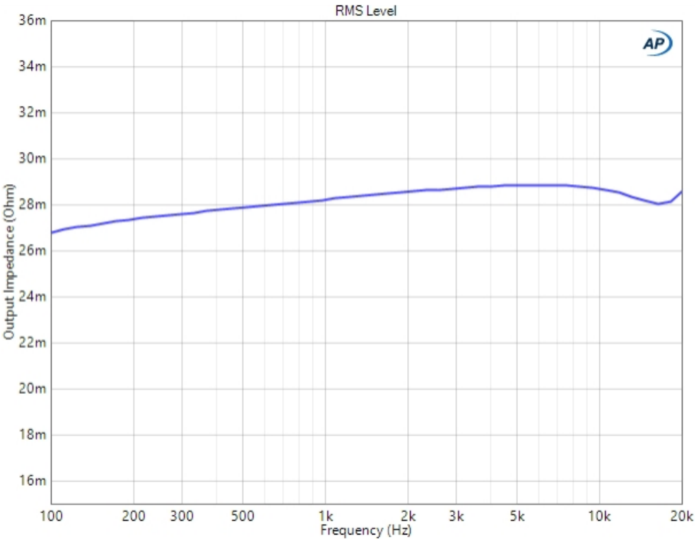
Figure 8: Measured voltage at output terminals while feeding 1Arms into the output of the amplifier at PCB
