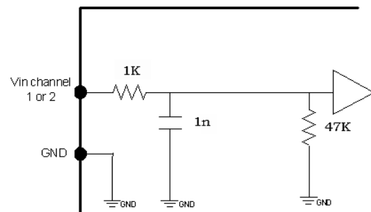
Figure 14: Single ended input buffer
