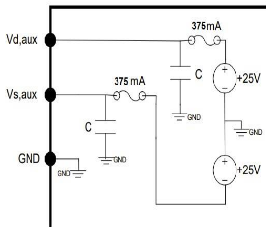
Figure 12: Auxiliary supply equivalent diagram
