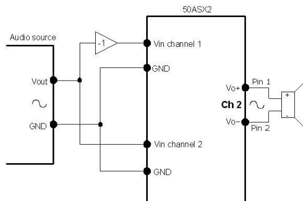
Figure 15: Wiring diagram for the BTL module
