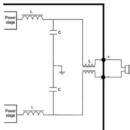
Figure 17: BTL output filter section
