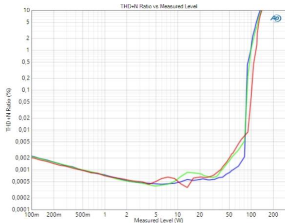
THD+N vs. Po at 100Hz(Blue), 1kHz(Green) and 6.67kHz(Red) 9) (8Ω), 230Vac/50Hz
