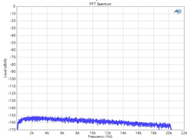
Idle noise (16K FFT). Residual = 25μV(A). (Relative to 50W into 4 ohm)
