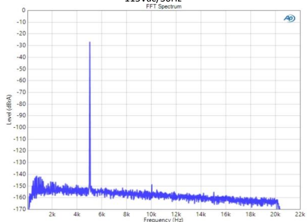
f = 5kHz. Po = 100mW. 4Ω loading. (Relative to 50W into 4 ohm)
