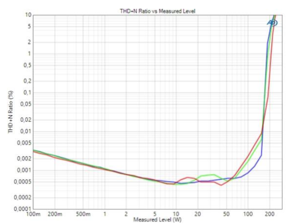
THD+N vs. Po at 100Hz(Blue), 1kHz(Green) and 6.67kHz(Red) 9) (4Ω), 115Vac/50Hz
